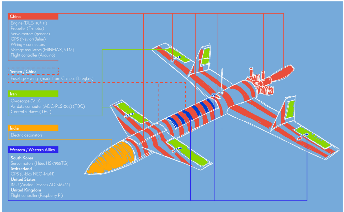
Figure 10. Houthi Qasf-2K composition by interdicted components.
